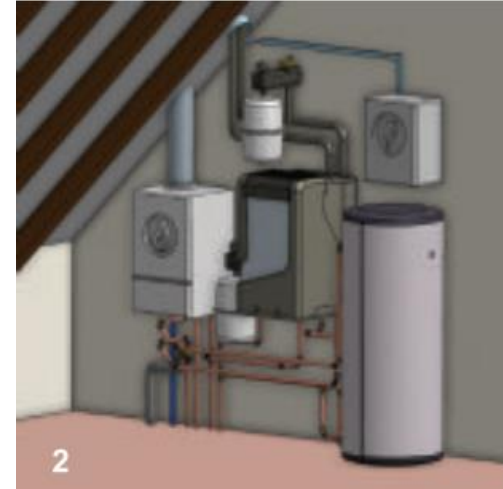
Hybride (CV+Wp+boiler)
